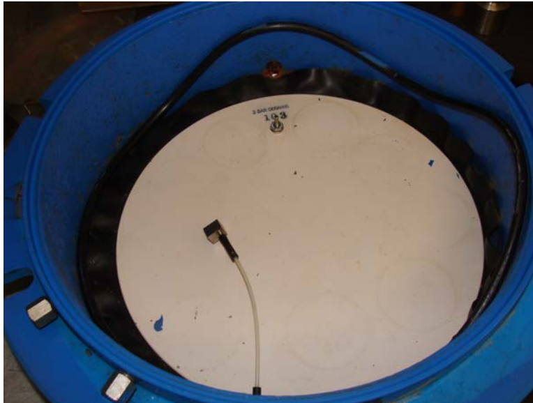
Figure A.8. Pressure plate extractor chamber for measuring soil moisture and potential.
